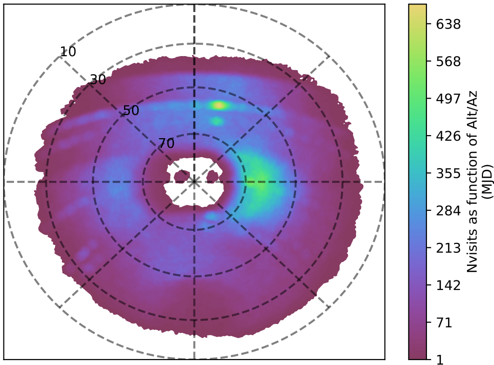
weather_cloudso20v3.4_10yrs u band: Nvisits as function of Alt/Az
