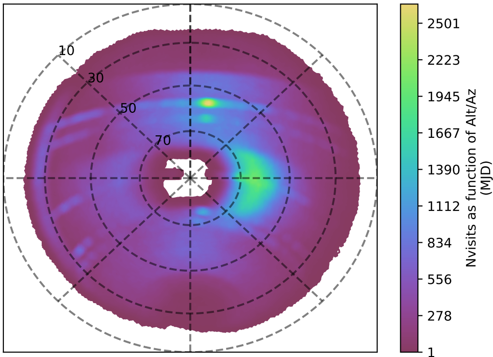
weather_cloudso20v3.4_10yrs r band: Nvisits as function of Alt/Az
