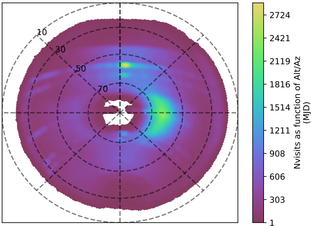
weather_cloudso20v3.4_10yrs i band: Nvisits as function of Alt/Az
