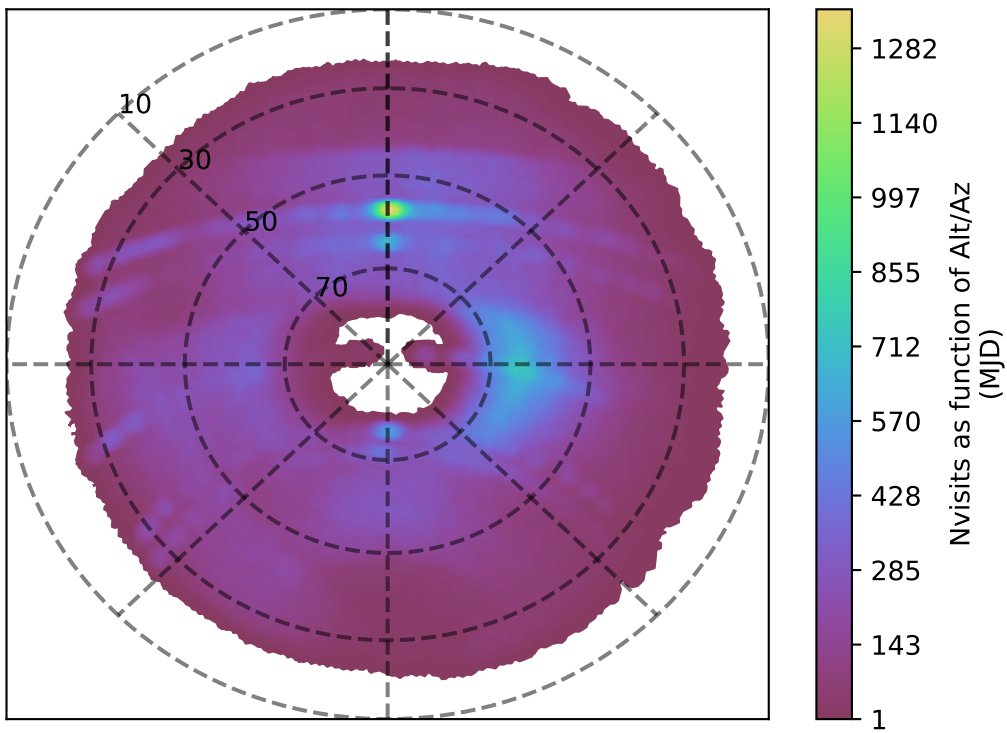
weather_cloudso20v3.4_10yrs g band: Nvisits as function of Alt/Az
