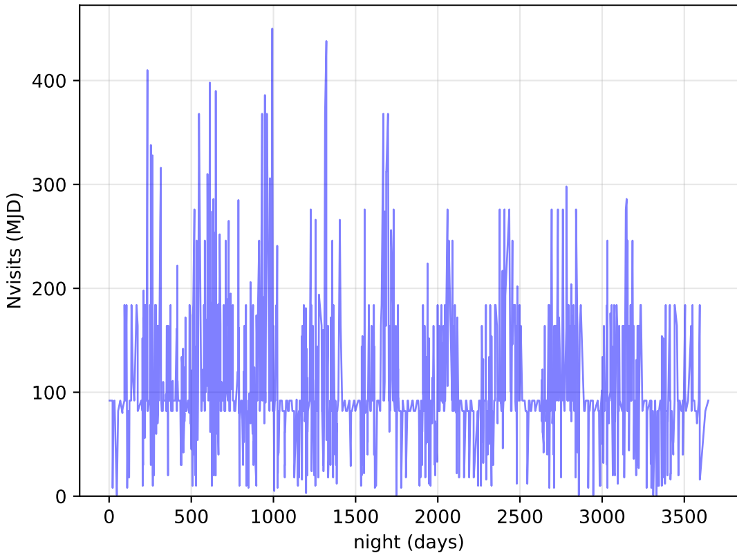
weather_cloudso20v3.4_10yrs DDF: Nvisits
