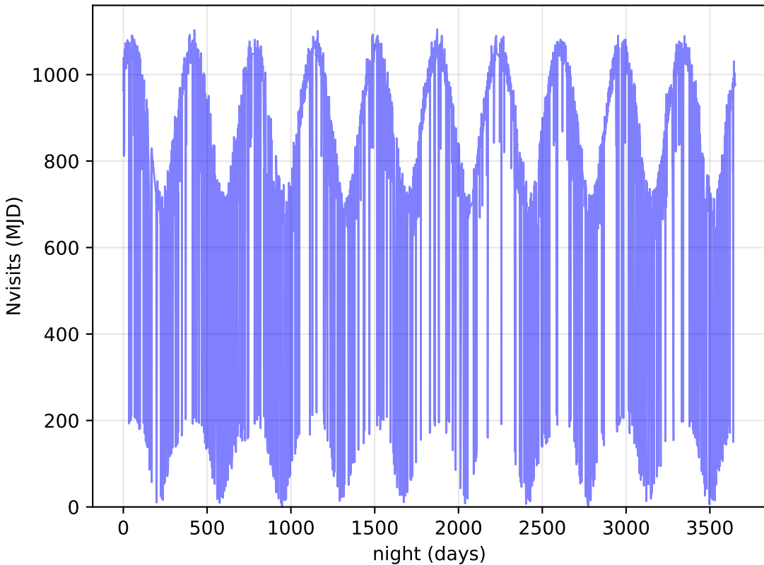
weather_cloudso20v3.4_10yrs All visits: Nvisits
