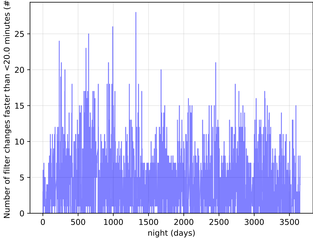
weather_cloudso20v3.4_10yrs Per Night: Number of filter changes faster than <20.0 minutes
