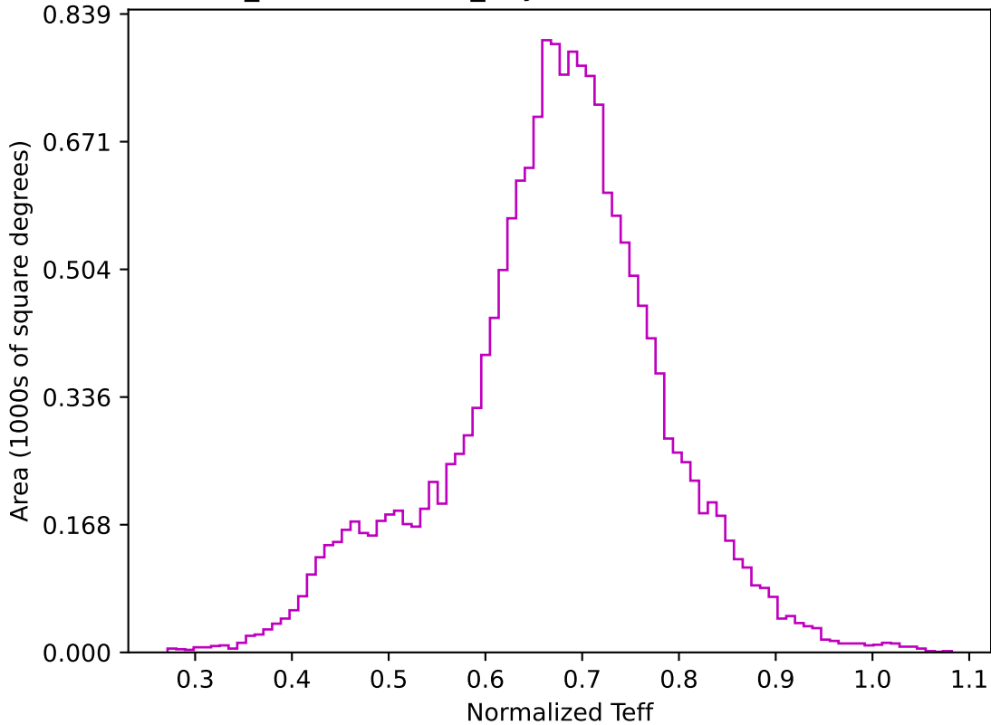
weather_cloudso20v3.4_10yrs WFD z band: Normalized Teff
