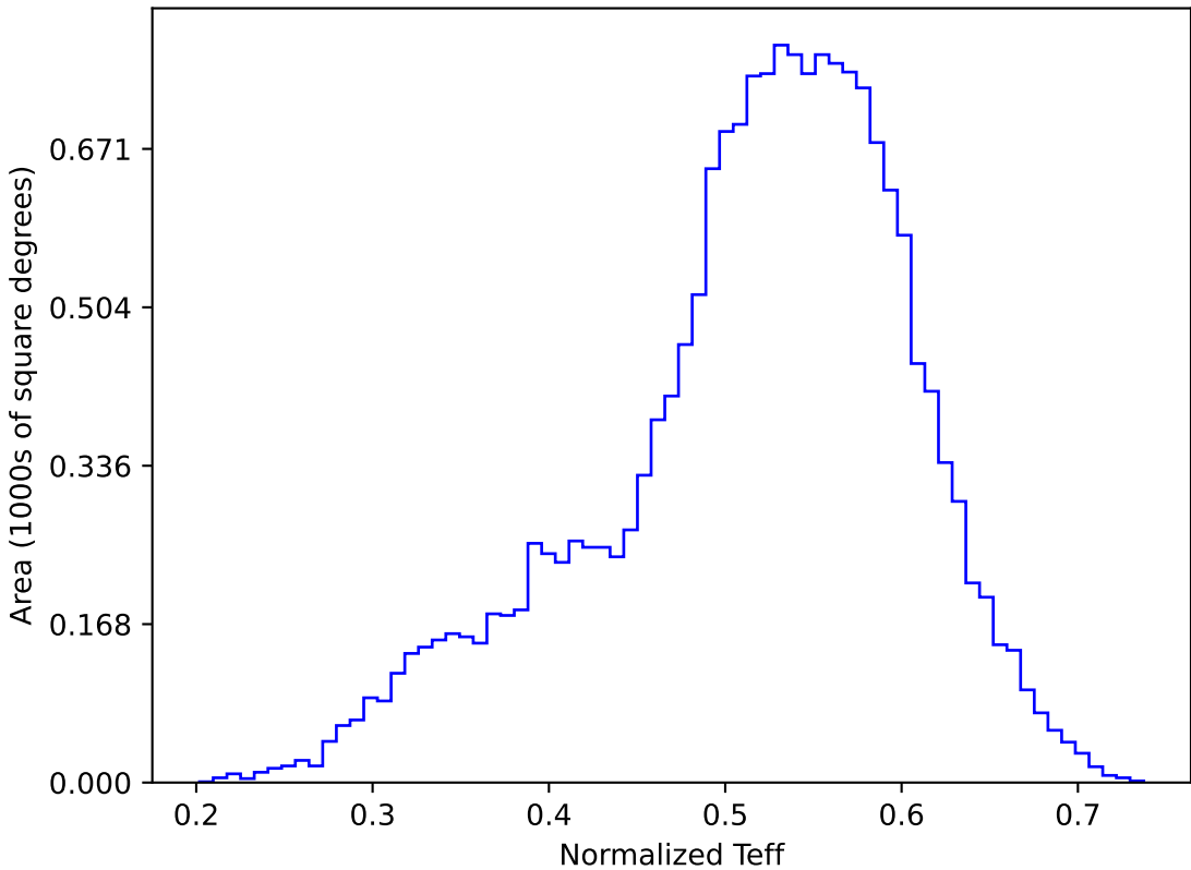
weather_cloudso20v3.4_10yrs WFD y band: Normalized Teff
