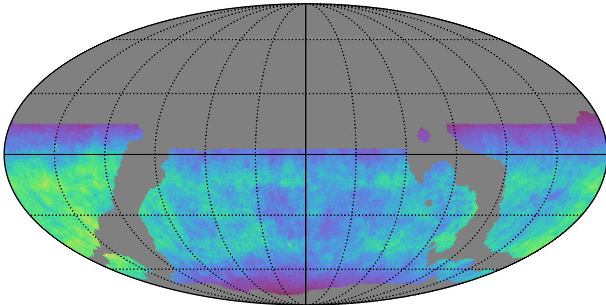
weather_cloudso20v3.4_10yrs WFD u band: Normalized Teff
