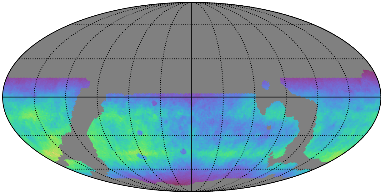
weather_cloudso20v3.4_10yrs WFD r band: Normalized Teff
