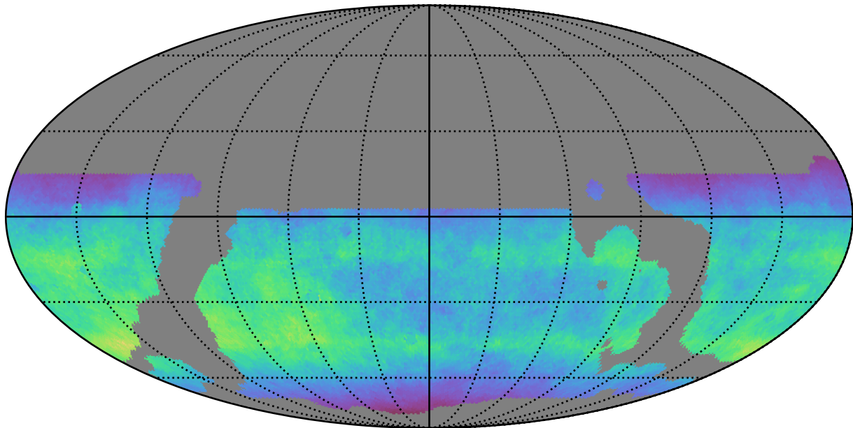
weather_cloudso20v3.4_10yrs WFD i band: Normalized Teff
