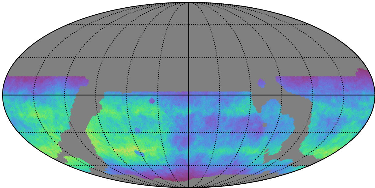
weather_cloudso20v3.4_10yrs WFD g band: Normalized Teff
