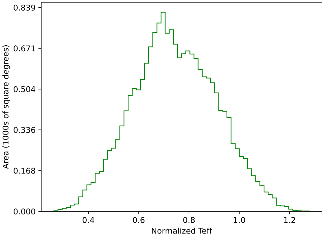
weather_cloudso20v3.4_10yrs WFD g band: Normalized Teff
