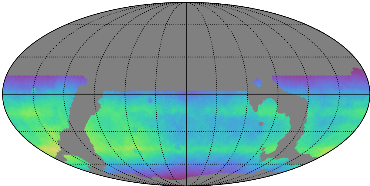
weather_cloudso20v3.4_10yrs WFD all bands: Normalized Teff
