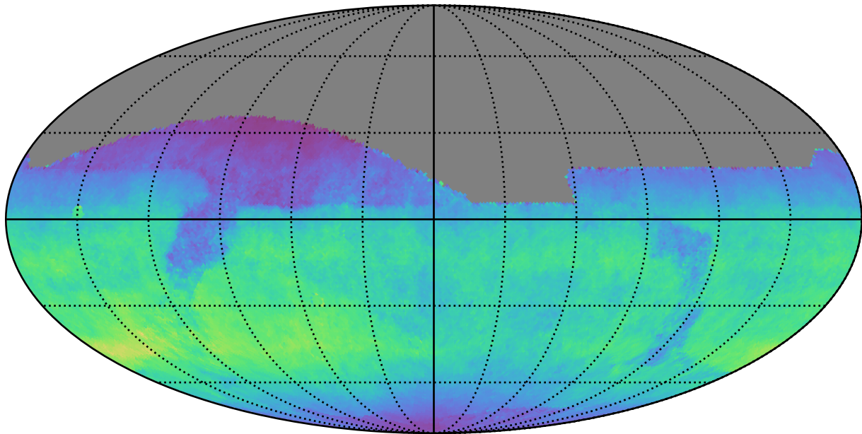
weather_cloudso20v3.4_10yrs All sky z band: Normalized Teff
