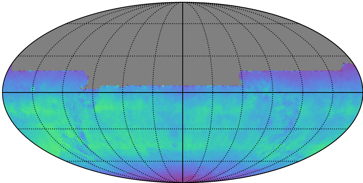
weather_cloudso20v3.4_10yrs All sky y band: Normalized Teff
