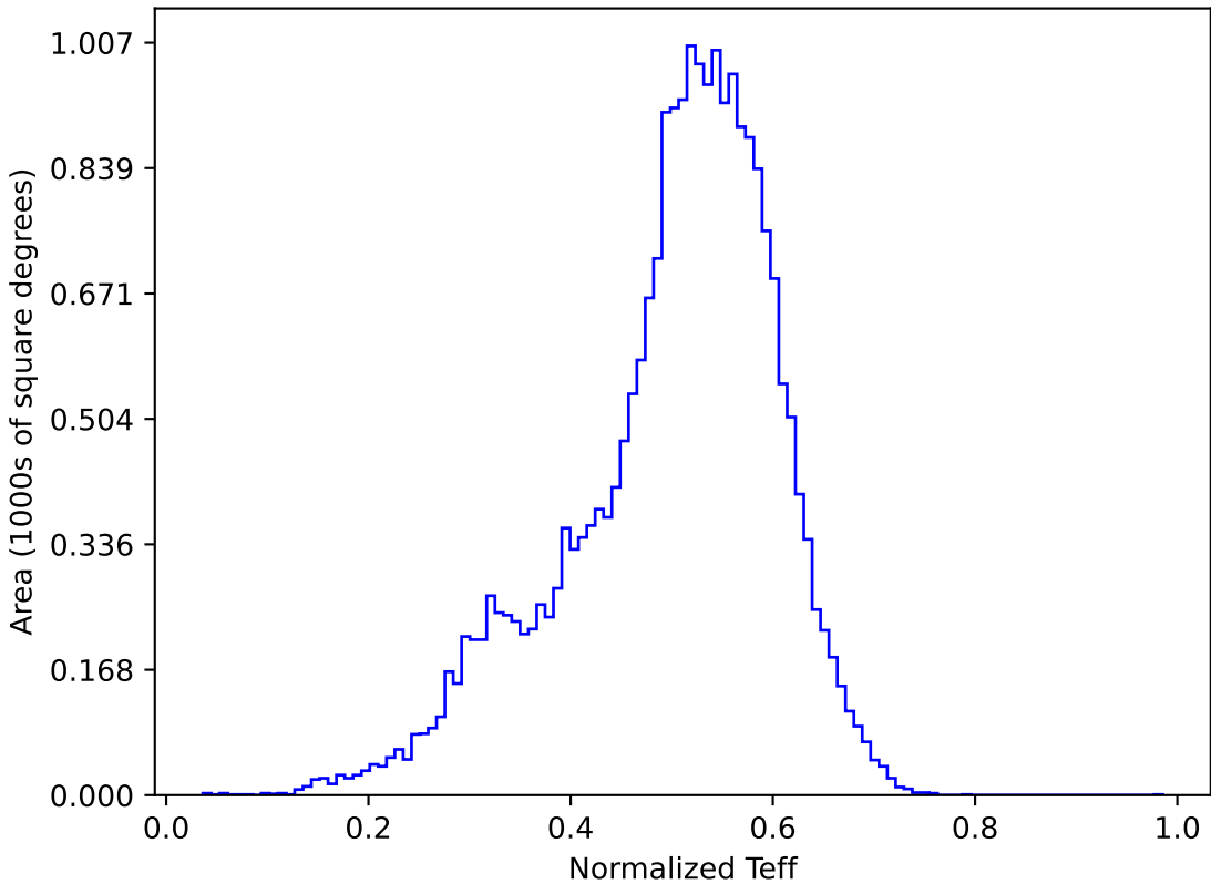
weather_cloudso20v3.4_10yrs All sky y band: Normalized Teff
