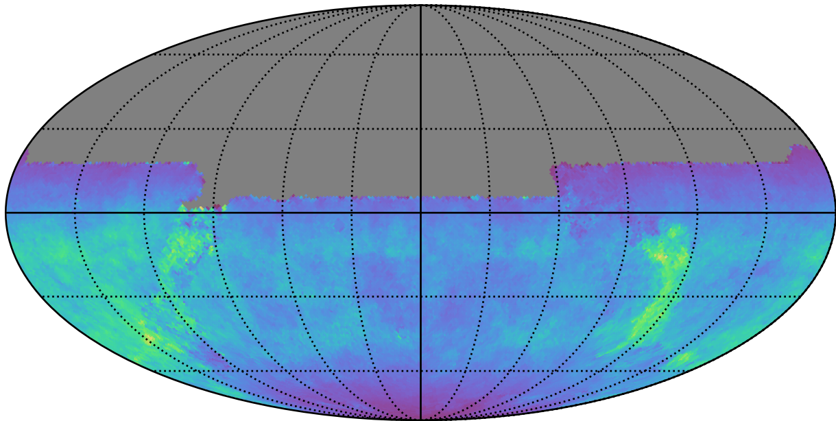
weather_cloudso20v3.4_10yrs All sky u band: Normalized Teff
