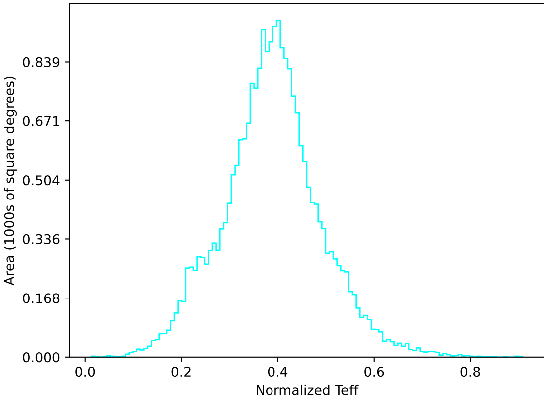
weather_cloudso20v3.4_10yrs All sky u band: Normalized Teff
