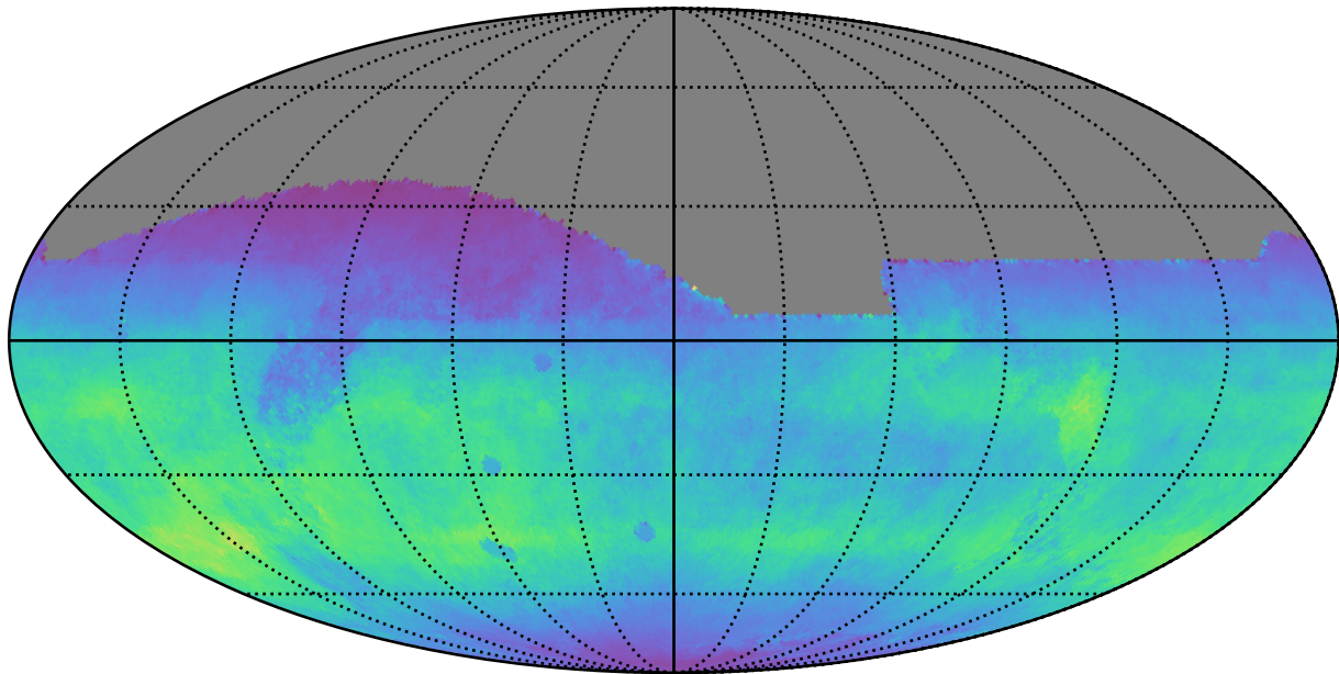
weather_cloudso20v3.4_10yrs All sky r band: Normalized Teff
