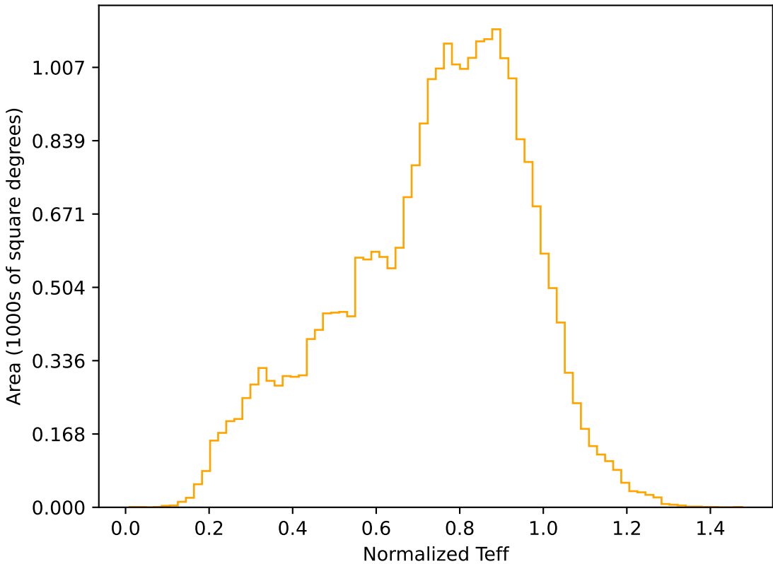
weather_cloudso20v3.4_10yrs All sky r band: Normalized Teff
