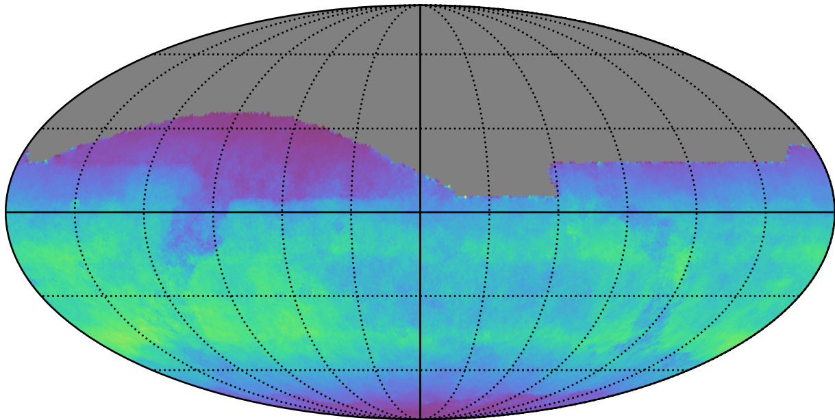
weather_cloudso20v3.4_10yrs All sky i band: Normalized Teff
