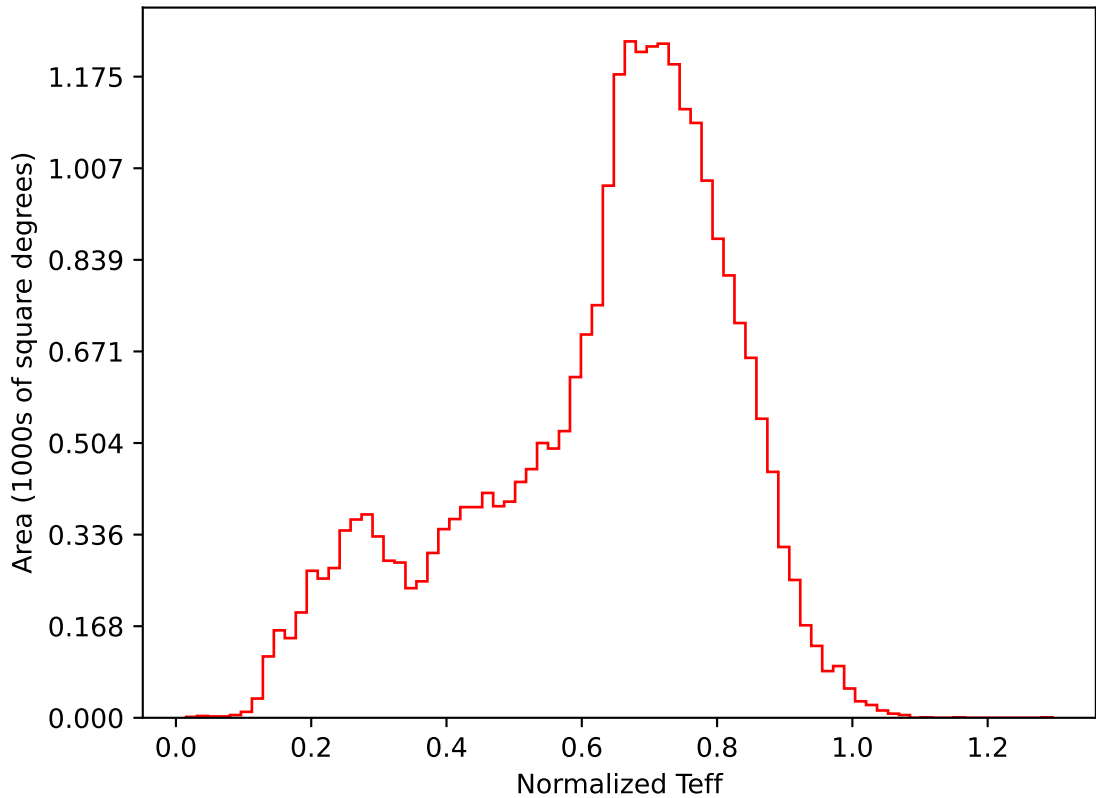
weather_cloudso20v3.4_10yrs All sky i band: Normalized Teff
