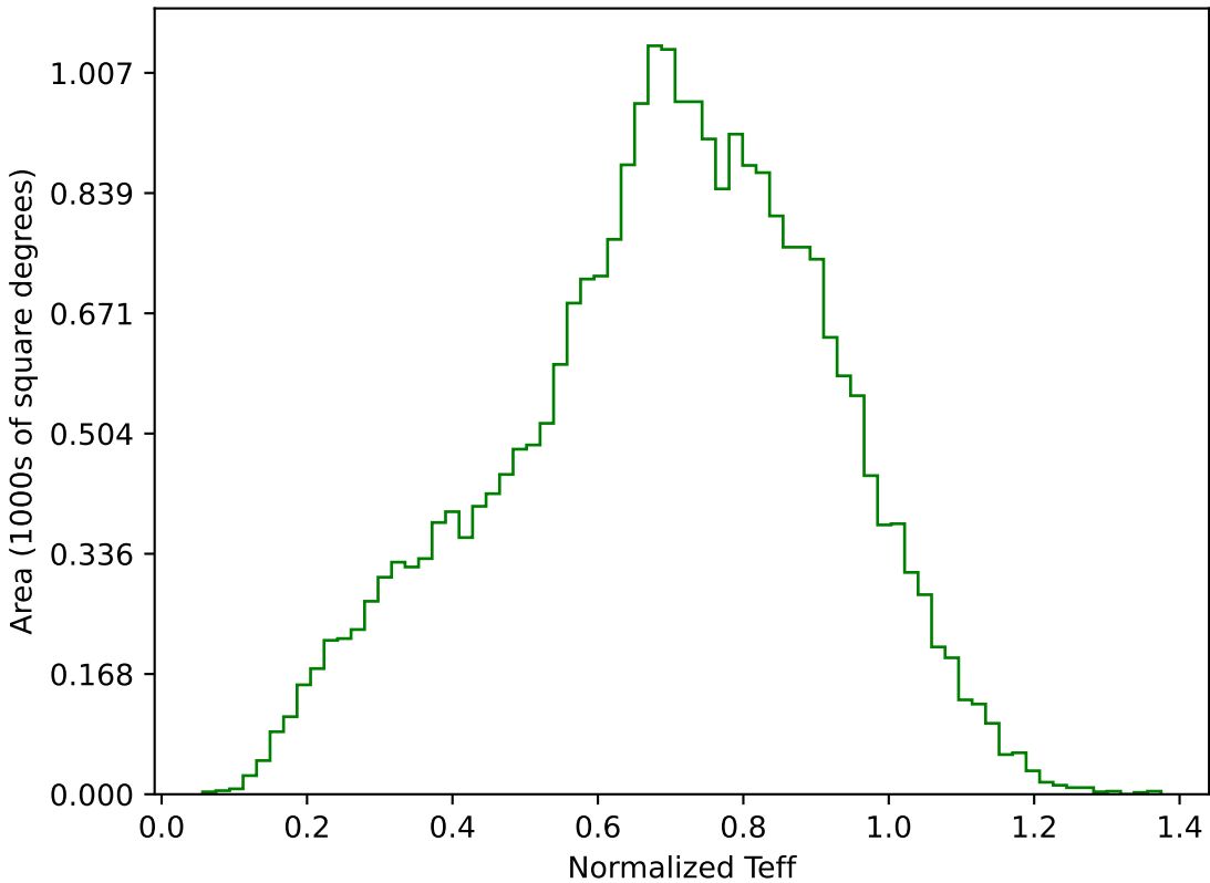
weather_cloudso20v3.4_10yrs All sky g band: Normalized Teff
