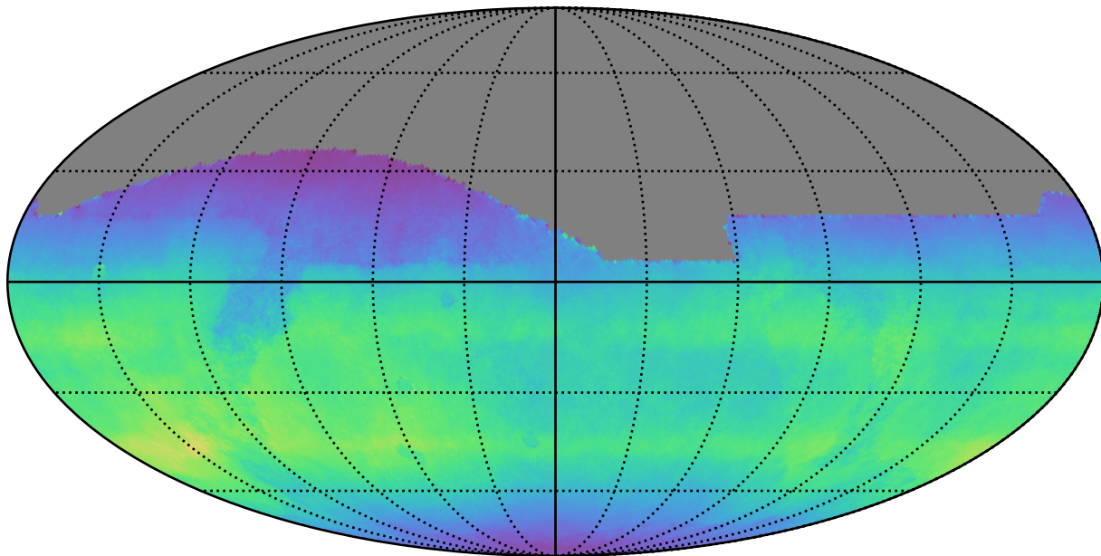
weather_cloudso20v3.4_10yrs All sky all bands: Normalized Teff
