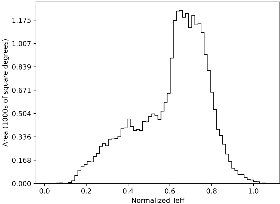
weather_cloudso20v3.4_10yrs All sky all bands: Normalized Teff
