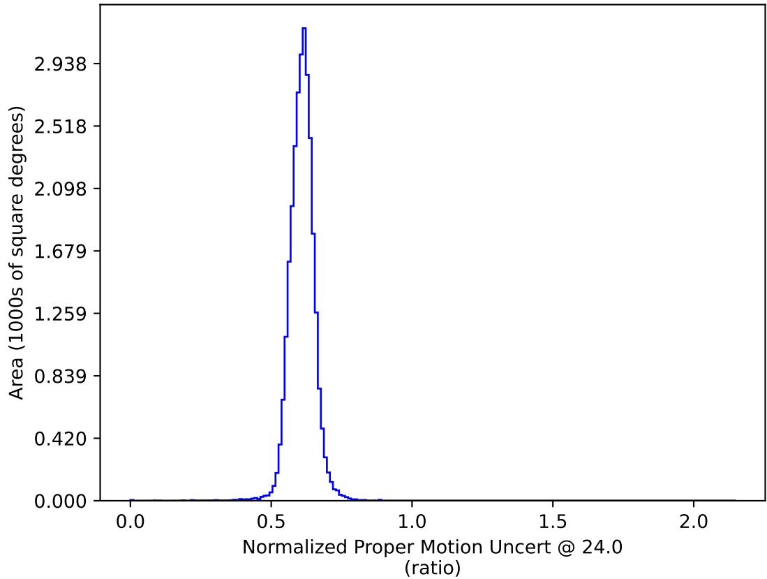
weather_cloudso20v3.4_10yrs All sky: Normalized Proper Motion Uncert @ 24.0
