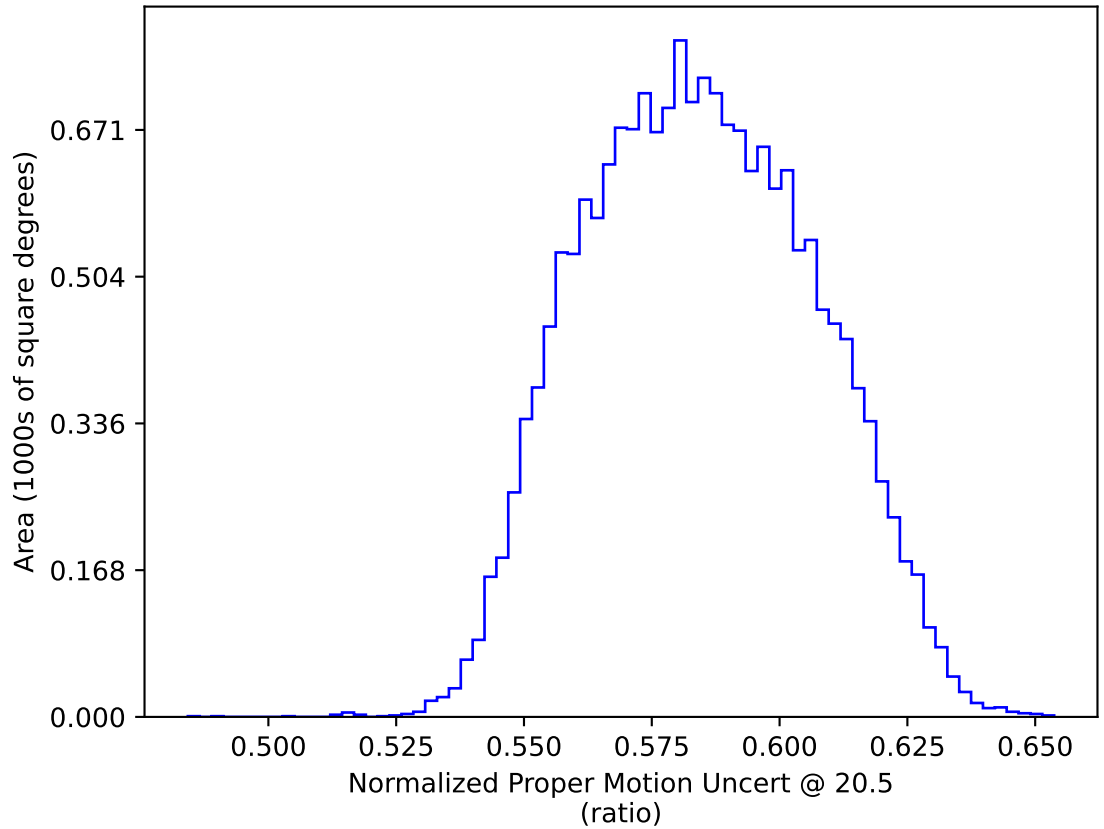
weather_cloudso20v3.4_10yrs WFD: Normalized Proper Motion Uncert @ 20.5
