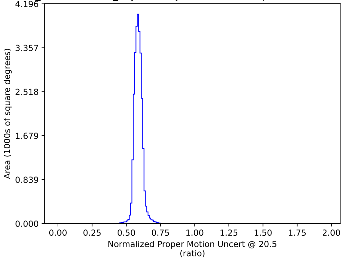
weather_cloudso20v3.4_10yrs All sky: Normalized Proper Motion Uncert @ 20.5
