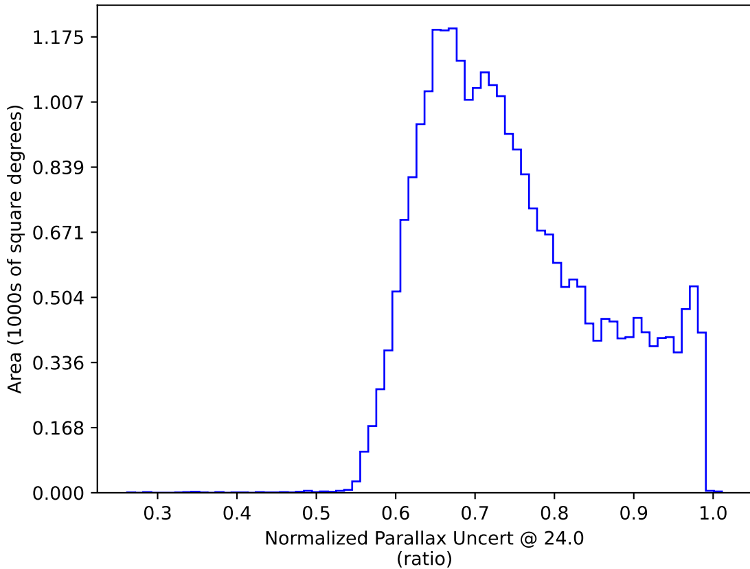
weather_cloudso20v3.4_10yrs All sky: Normalized Parallax Uncert @ 24.0
