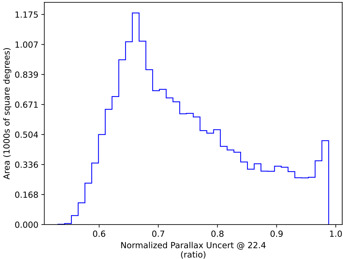
weather_cloudso20v3.4_10yrs WFD: Normalized Parallax Uncert @ 22.4
