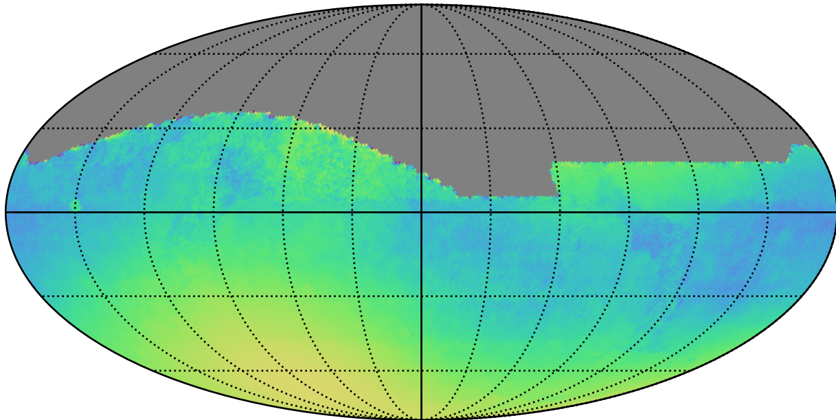
weather_cloudso20v3.4_10yrs All sky: Normalized Parallax Uncert @ 22.4
