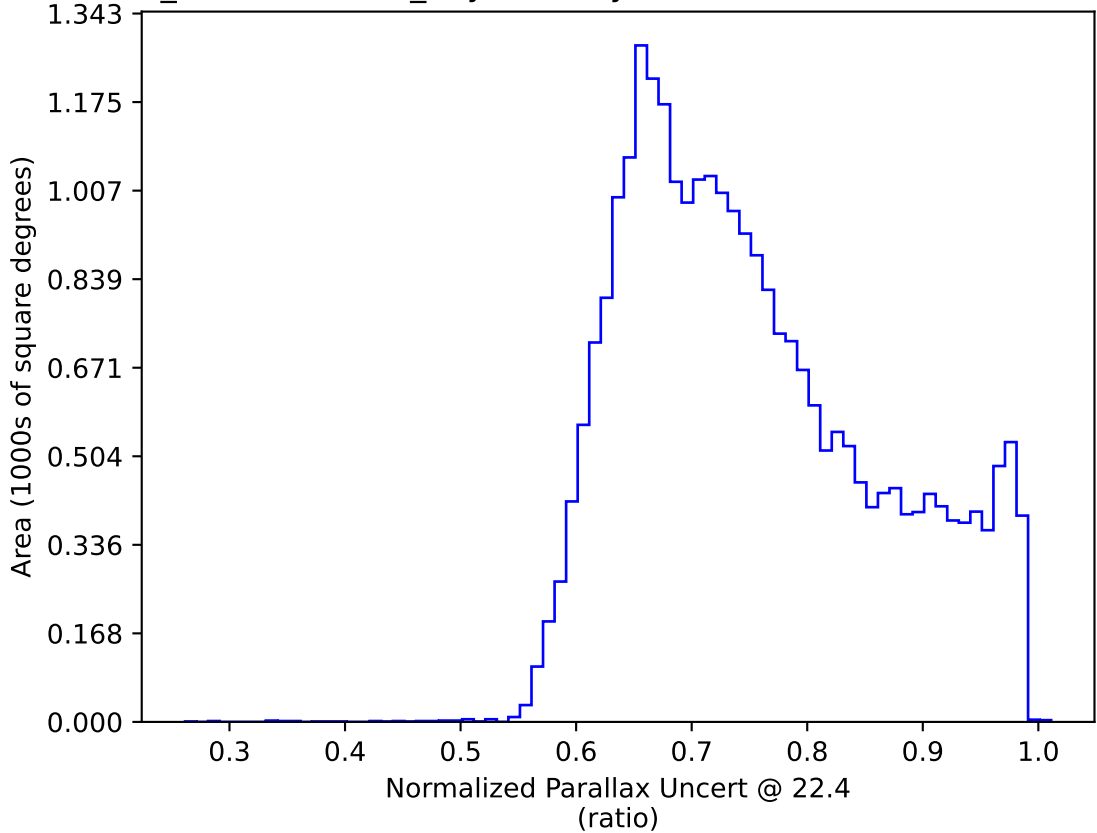
weather_cloudso20v3.4_10yrs All sky: Normalized Parallax Uncert @ 22.4
