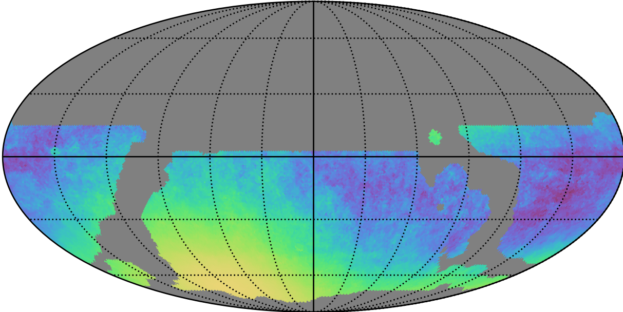
weather_cloudso20v3.4_10yrs WFD y band only: Normalized Parallax Uncert @ 21.3
