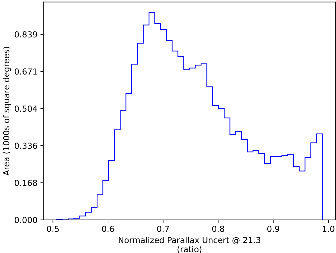
weather_cloudso20v3.4_10yrs WFD y band only: Normalized Parallax Uncert @ 21.3
