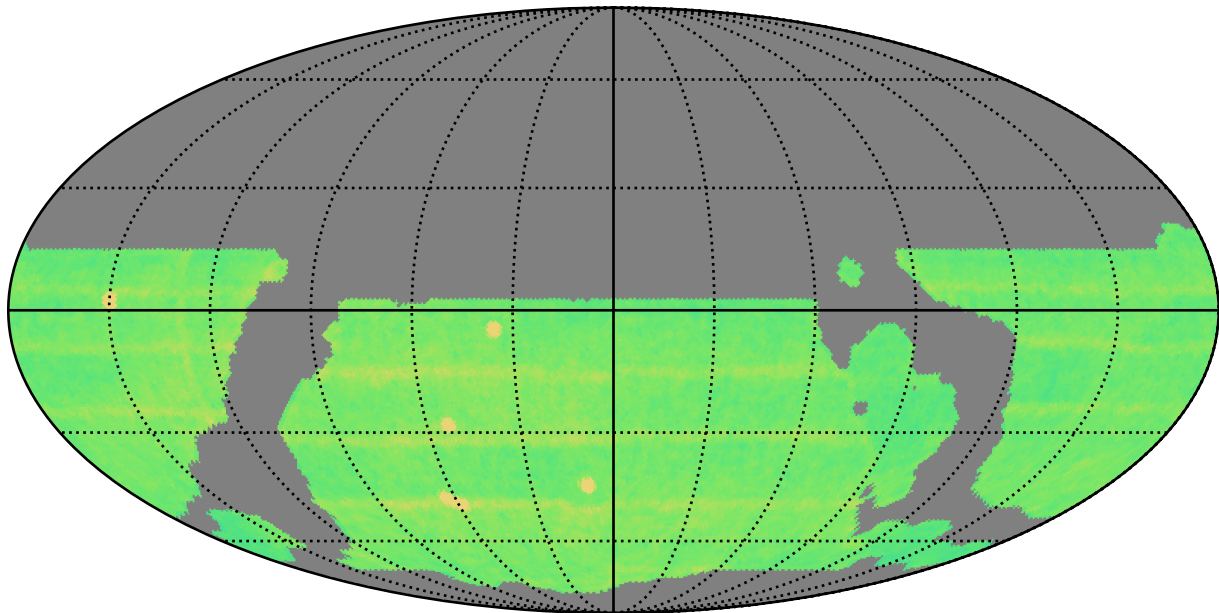
weather_cloudso20v3.4_10yrs WFD all bands: N Unique Nights
