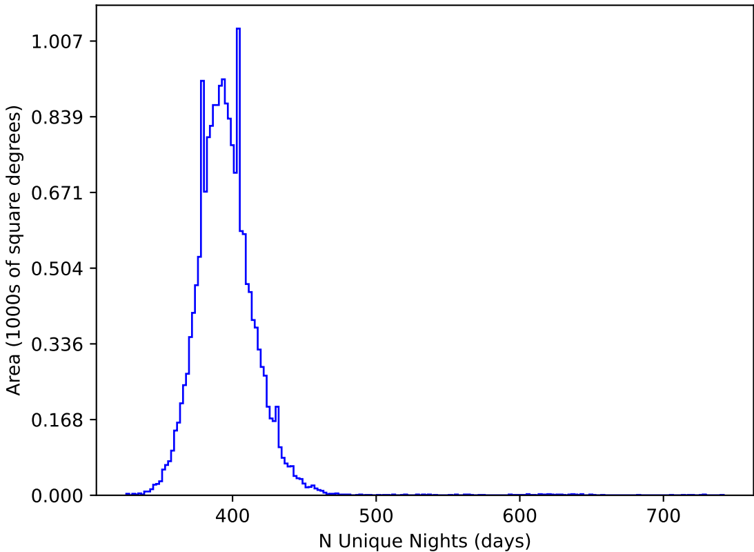
weather_cloudso20v3.4_10yrs WFD all bands: N Unique Nights
