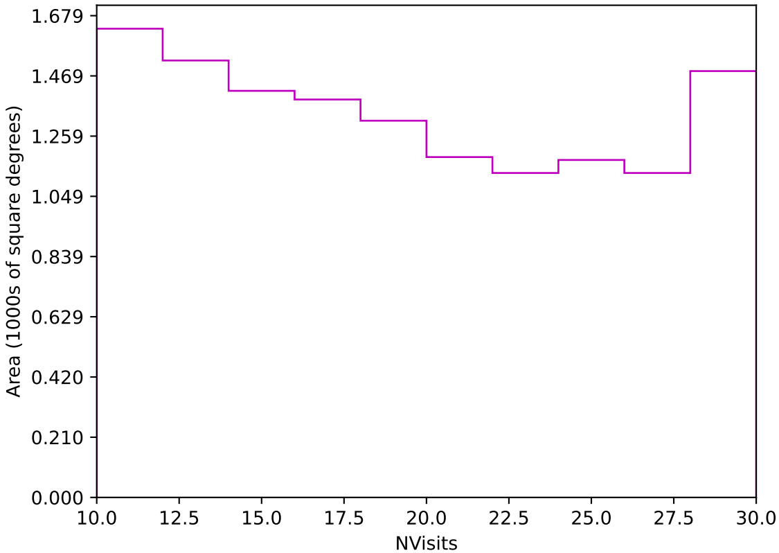
weather_cloudso20v3.4_10yrs Yr 3-4 z band: NVisits
