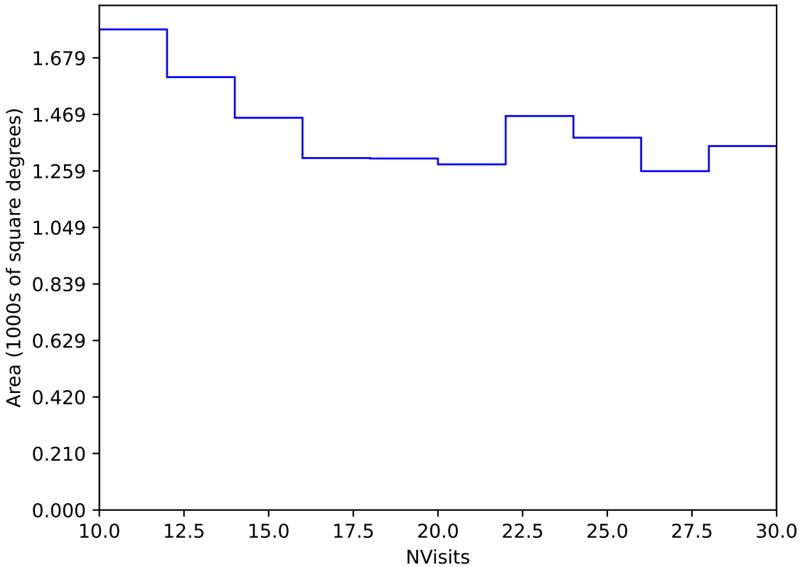
weather_cloudso20v3.4_10yrs Yr 3-4 y band: NVisits
