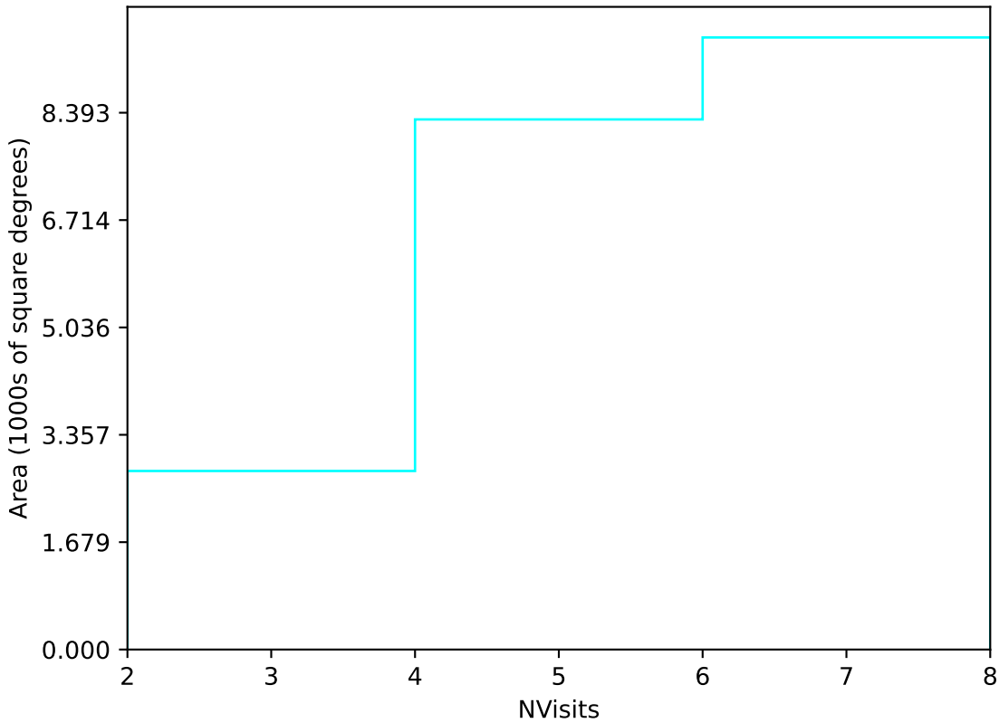
weather_cloudso20v3.4_10yrs Yr 1 u band: NVisits
