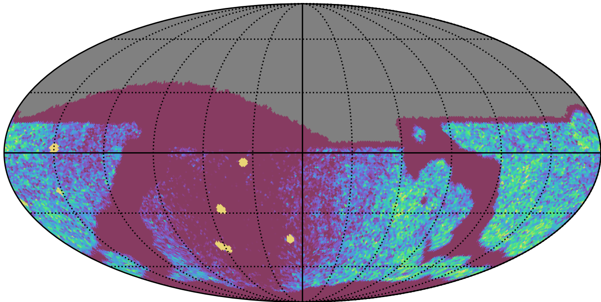
weather_cloudso20v3.4_10yrs Yr 1 all bands: NVisits
