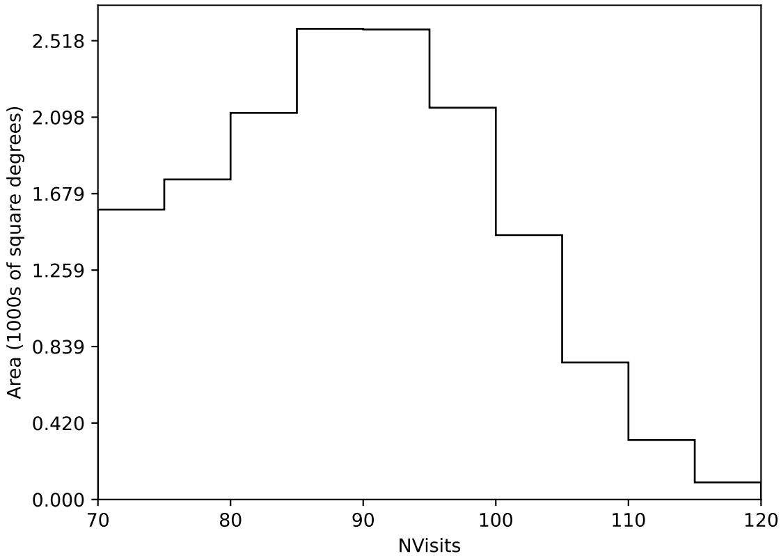
weather_cloudso20v3.4_10yrs Yr 1 all bands: NVisits
