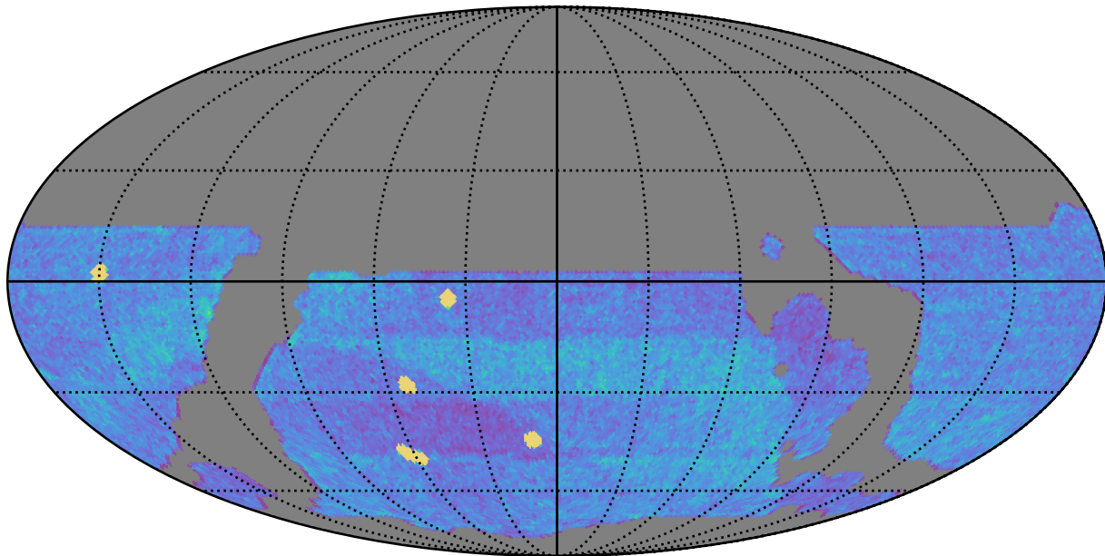
weather_cloudso20v3.4_10yrs WFD all bands: NVisits
