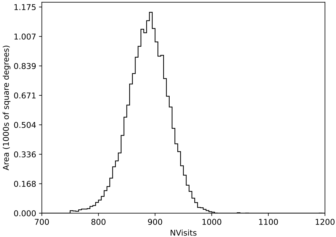
weather_cloudso20v3.4_10yrs WFD all bands: NVisits
