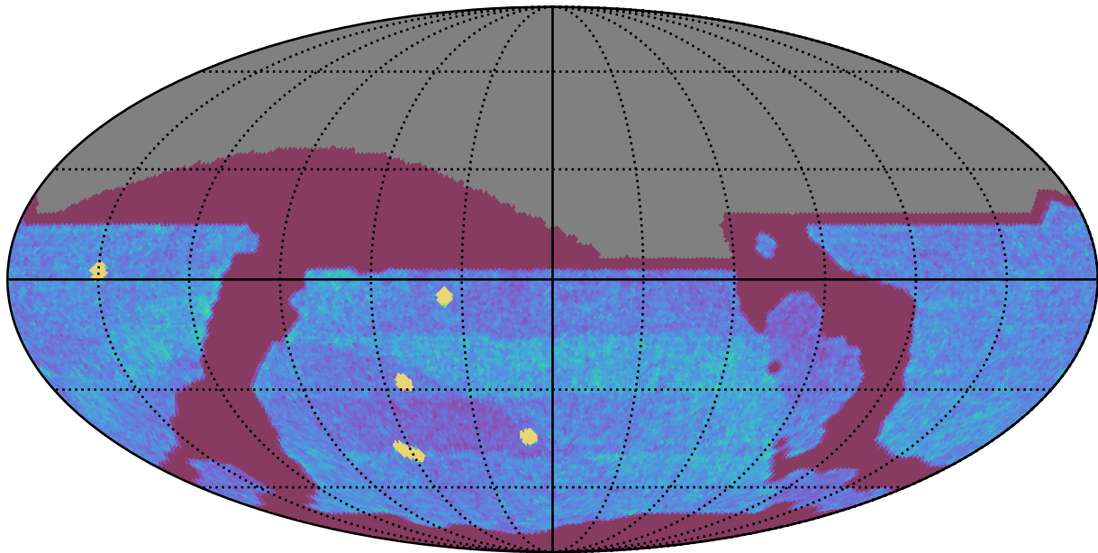
weather_cloudso20v3.4_10yrs All sky all bands: NVisits
