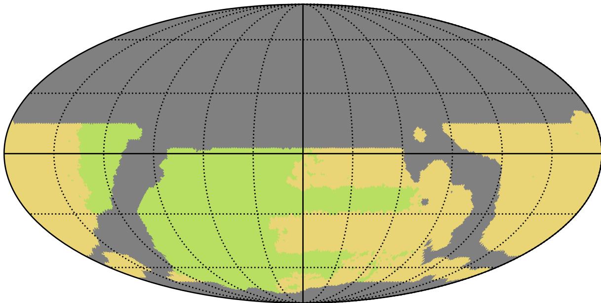
weather_cloudso20v3.4_10yrs WFD all bands: NSeasons
