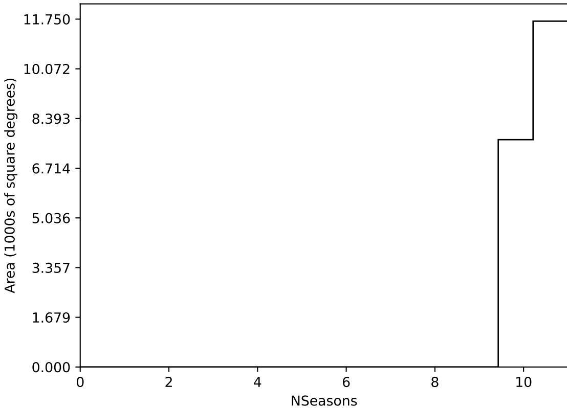
weather_cloudso20v3.4_10yrs WFD all bands: NSeasons
