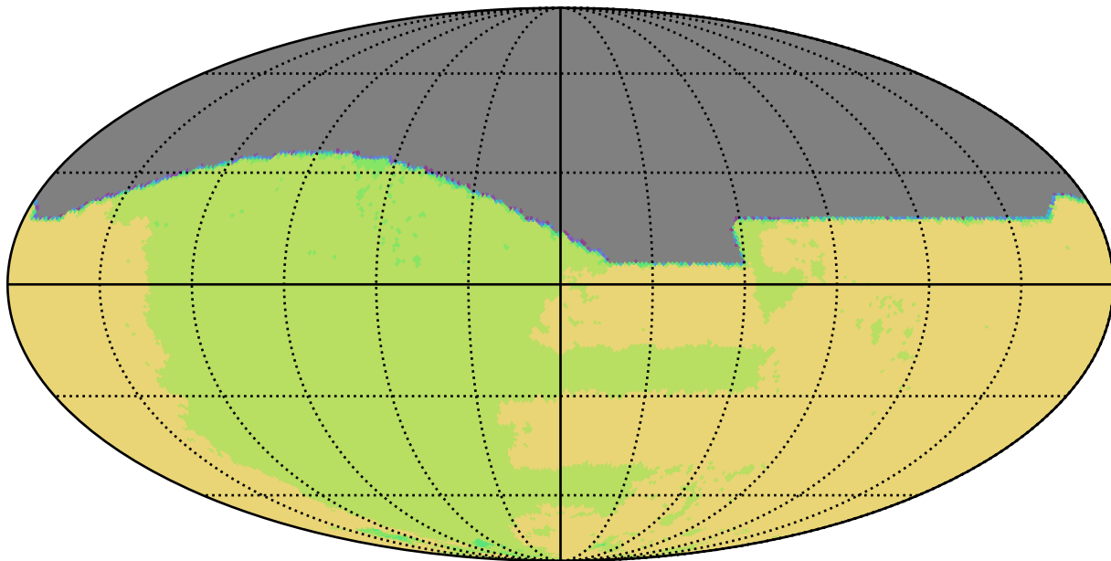
weather_cloudso20v3.4_10yrs All sky all bands: NSeasons
