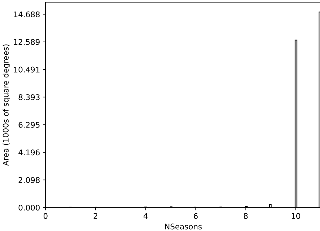
weather_cloudso20v3.4_10yrs All sky all bands: NSeasons
